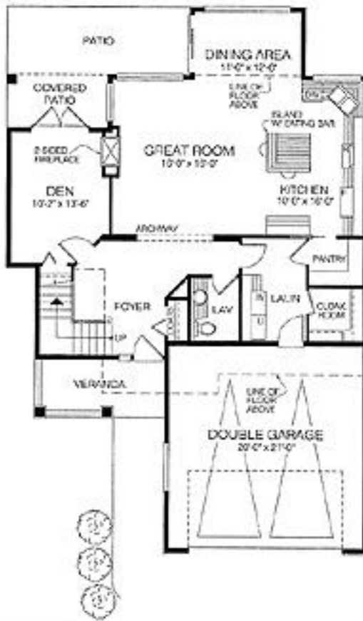
MAIN FLOOR PLAN 1074 SQ. FT. (99.8 M 2 ) 9'-0" CEILING HEIGHT
